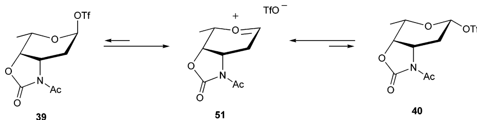
FIGURE 5. Equilibrium between the oxacarbenium ion ( 51 ) and glycosyl triflate intermediates ( 39 and 40 ) produced from treatment of thioglycoside 22 with BSP and \text{Tf}_2\text{O} . The flattening of the pyranose ring induced by the carbamate moiety would be expected to reduce the torsional barrier leading to 51 .
