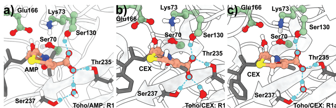
Fig. 2 Conformations of R1 reactant states. The conformations of (a) Toho/AMP: R1; (b) Toho/CEX: R1; (c) Toho/CEX: R1a. The hydrogen bonding interactions are noted as blue dashed lines.
