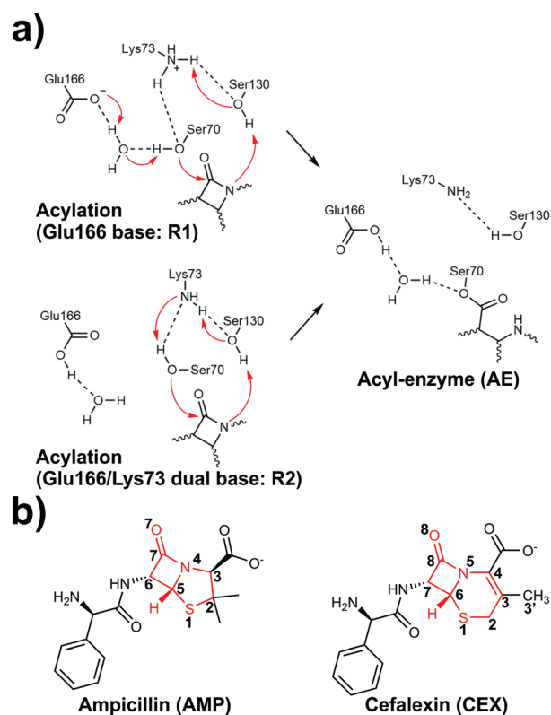
Fig. 1 Mechanisms of acylation in AS \beta LS and structures of the model substrates. (a) The general mechanism of \beta -lactam acylation mediated by AS \beta L; (b) structures of ampicillin (AMP) and cefalexin (CEX).
