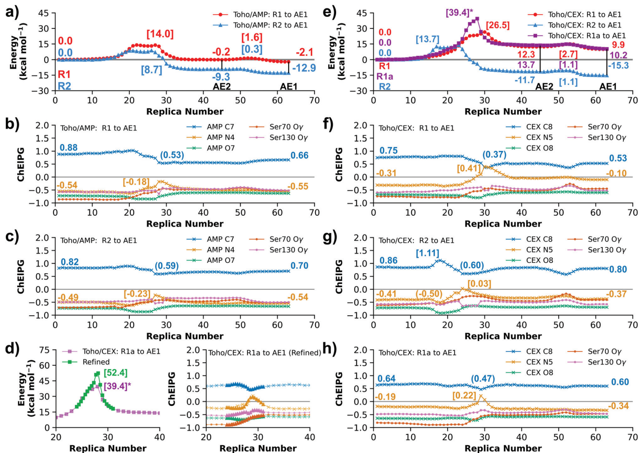
Fig. 3 Energy profiles and the ChEIPG charges of key atoms along the acylation pathways in Toho-1 hydrolysis. (a) The acylation profiles of Toho/AMP; the ChEIPG charges along (b) the Toho/AMP: R1 to AE1 pathway, and (c) the Toho/AMP: R2 to AE1 pathway; (d) the energy profile and the ChEIPG charge profiles of the refined Toho/CEX: R1a to AE1 pathways, which is calculated from inserting 18 replicas between replica 24 and 31 (see ESI†); (e) the acylation profiles of Toho/CEX; the ChEIPG charges along (f) the Toho/CEX: R1 to AE1 pathway, (g) the Toho/CEX: R2 to AE1 pathway, and (h) the Toho/CEX: R1a to AE1 pathway. The vertical black solid lines in (a) and (d) indicate the location of AE1 and AE2. Numbers in parentheses and brackets denote the local minimum and maximum values of important states along the reaction path. Note that only ChEIPG charge values of \beta -lactam carbonyl carbon (blue) and nitrogen (orange) are shown in (b), (c), (f), (g) and (h). See also Tables S3–S7† for detailed replica-wise energy components and ChEIPG charges on key atoms.
