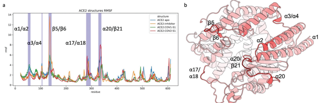
Fig. 2 Root Mean Squared Fluctuation (RMSF) analysis of ACE2 PD in different systems. (a) RMSF plot of ACE2 PD residues C \alpha for ACE2:apo, ACE2:inhibitor, ACE2:COV1-S1, and ACE2:COV2-S1. (b) ACE2 PD fluctuation trends in its apo form. The color gradient from white to red represents the degree of flexibility from low to high, respectively. Protein rendered with 3D Protein Imaging. 74
