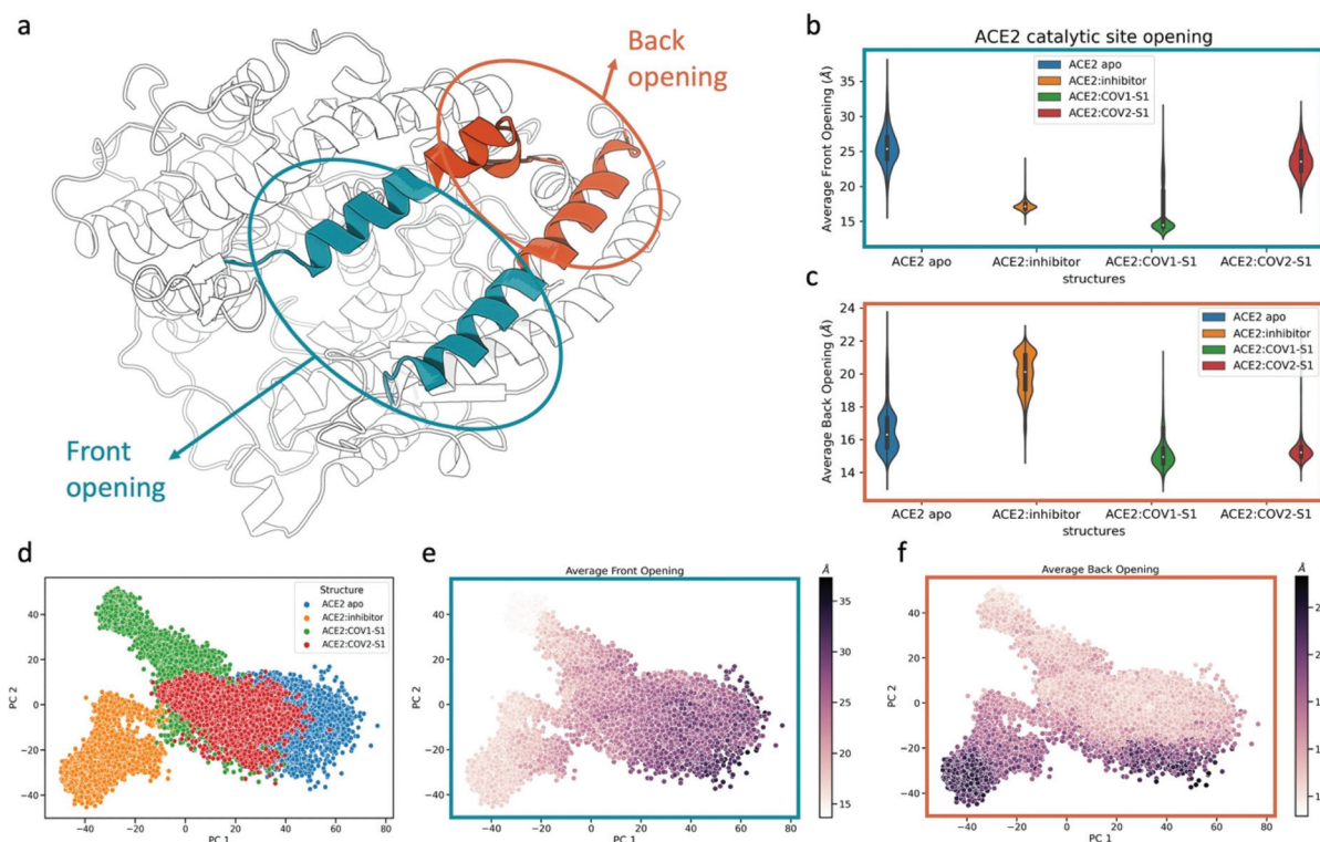
Fig. 3 Conformational space of ACE2 PD related to the front and back openings of its binding site in different states. (a) Structure of ACE2 peptidase domain (PD). The helices involving the front and back opening are colored in blue and orange, respectively. The helices involved are the \alpha 2 and \alpha 4 (Table S1†). (b) Distance distributions of the front opening in the different ACE2 states. The distances reported are the average distance between the residues 69 to 84 of the \alpha 2 and the residues 101 to 116 of \alpha 4 . (c) Distance distributions of the back opening in the different ACE2 structures. The distances reported are the average distance between the residues 53 to 68 of the \alpha 2 and the residues 117 to 132 of \alpha 4 . (d) Projection of each state onto the conformational space represented by the first two components of principal component analysis. Each data point represents a frame (conformation) of ACE2 PD. Colored scheme: blue for ACE2 apo, orange for ACE2:inhibitor, green for ACE2:COV1-S1, red for ACE2:COV2-S1. (e) Projection of conformational space explored using the first two components of principal component analysis. The data points are colored based on the value of average distance between the carbons of the helices at the entrance of ACE2 binding site (front opening). (f) Projection of conformational space explored using the first two components of principal component analysis. The data points are colored based on the value of average distance between the carbons of the helices at the back of ACE2 binding site (back opening). Points are colored from light to dark for small to large distances, respectively. Protein rendered with 3D Protein Imaging. 74
