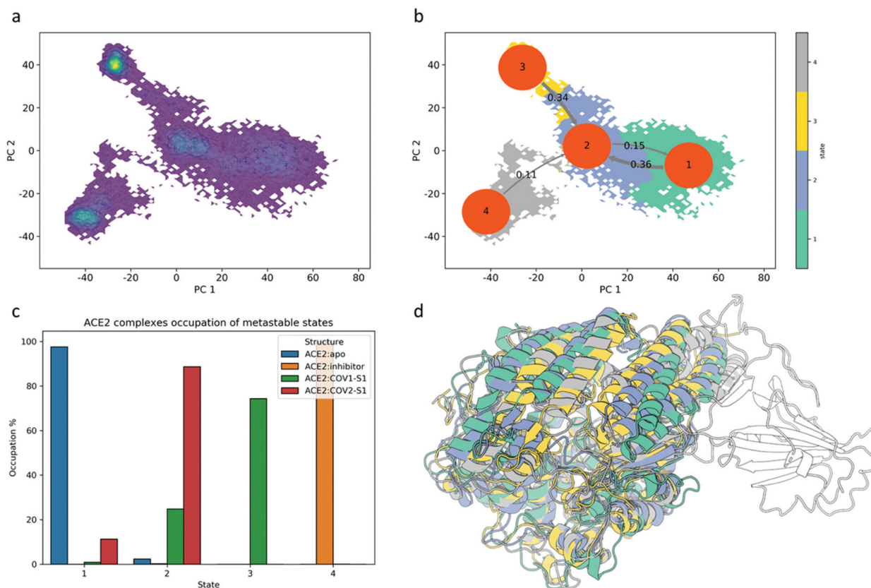
Fig. 4 Identification and analysis of ACE2 PD macrostates using kinetical clustering. The clustering method used is PCCA+ on the assumption that conformations belonging to the same macrostate interconvert rapidly compared to transitioning to another macrostate. (a) Visualization of high-density areas on the ACE2 conformational space, which correspond to energy minima. (b) Visualization of PCCA+ macroclusters on the projected conformational space. The flux between the states is included as inverse of mean time passage. The choice of using four clusters was confirmed from the plot of implied timescales at different lag times of our Markov state model (Fig S3†). (c) ACE2 PD occupation of the different metastable states. (d) Overlap of the ACE2 PB domain of the representative structures for the four macrostates identified. Macrostates representative structures are colored based on PCCA clustering. Protein rendered with 3D Protein Imaging. 74
