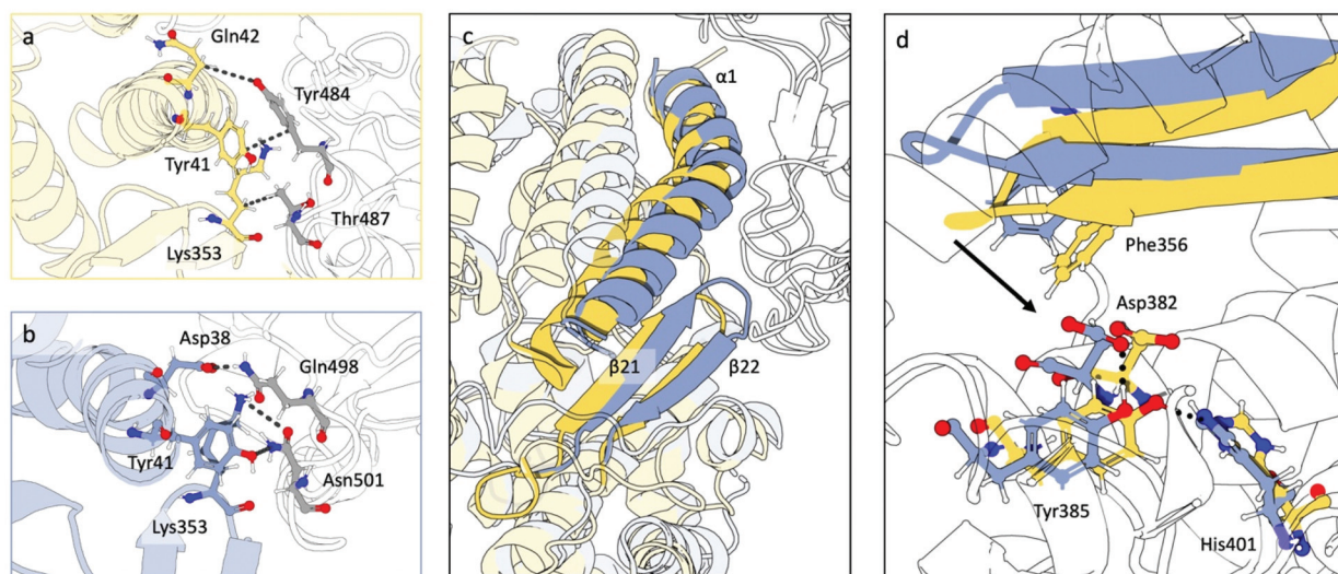
Fig. 7 Interaction between coronavirus S1 RBD fragments and ACE2 PD via contact analysis. (a) Contact analysis between the residues in \alpha 1 , \beta 21 , and \beta 22 of ACE2 PD and the SARS-CoV-1 S1 RBD residues Tyr484 and Thr487. Residues in yellow belong to ACE2, residues in grey belong to viral spike S1 RBD fragment. Contacts less than 4 Å for more than 50% of the frames were shown. From the contacts shown only a \pi -stacking interaction was found as energetically favored interaction. (b) Contact analysis between the residues in \alpha 1 , \beta 21 , and \beta 22 of ACE2 PD and the SARS-CoV-2 spike S1 RBD residues Gln498 and Asn501. Residues in blue belong to ACE2, residues in grey belong to viral spike fragment. Contacts less than 4 Å for more than 50% of the frames were shown. In this case, a strong network of energetically favorable interaction was identified. The RBD residues considered differ between the two coronaviruses spikes. (c) Details of the overlap of ACE2:COV1-S1 (in yellow) and ACE2:COV2-S1 (in blue). The secondary structures represented are \alpha 1 , \beta 21 , and \beta 22 . (d) Illustration of the effects of \beta 21 and \beta 22 shift on residues involved in the allosteric path. Protein rendered with 3D Protein Imaging. 74
